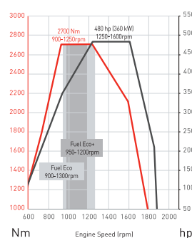
DE13 TC - 480 hp
