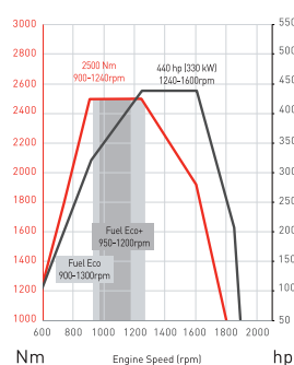
DE13 TC - 440 hp
